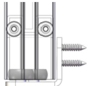
SIDE VIEW BOTTOM ROLLER
