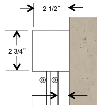
SIDE VIEW BOTTOM ROLLER
